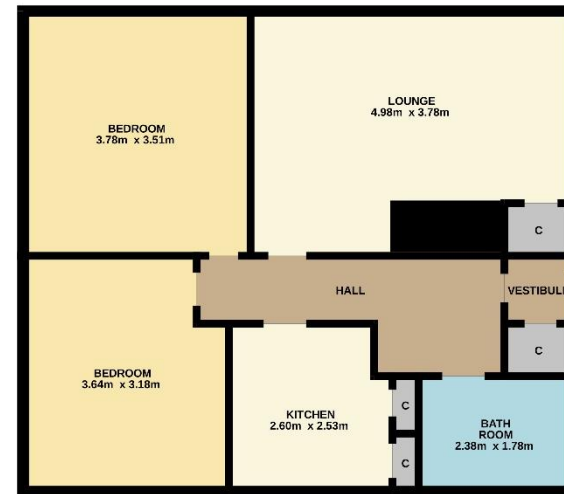
FIRST FLOOR 67.0 sq.m. approx.
