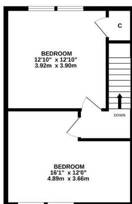
1ST FLOOR
