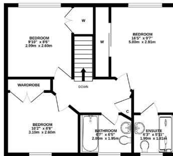
1ST FLOOR
