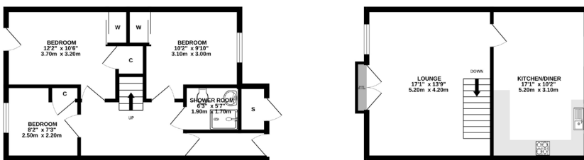
GROUND FLOOR
