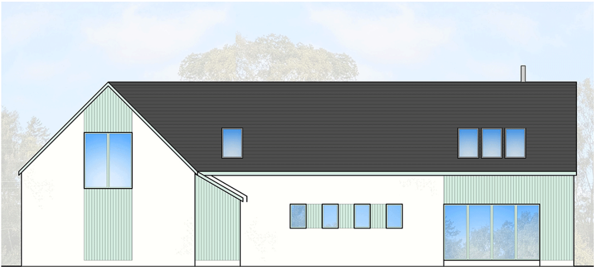
North Elevation
