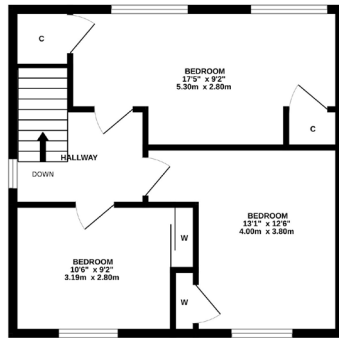
1ST FLOOR
