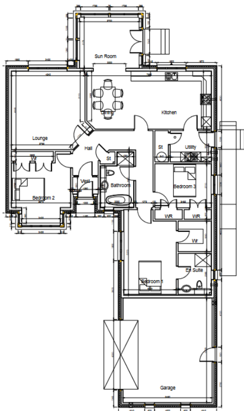
Ground Floor Plan 1:50
